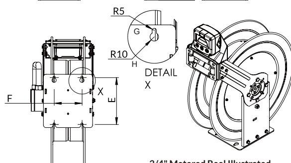
- 3/4" Metered Reel Illustrated - Dimensions are in mm
